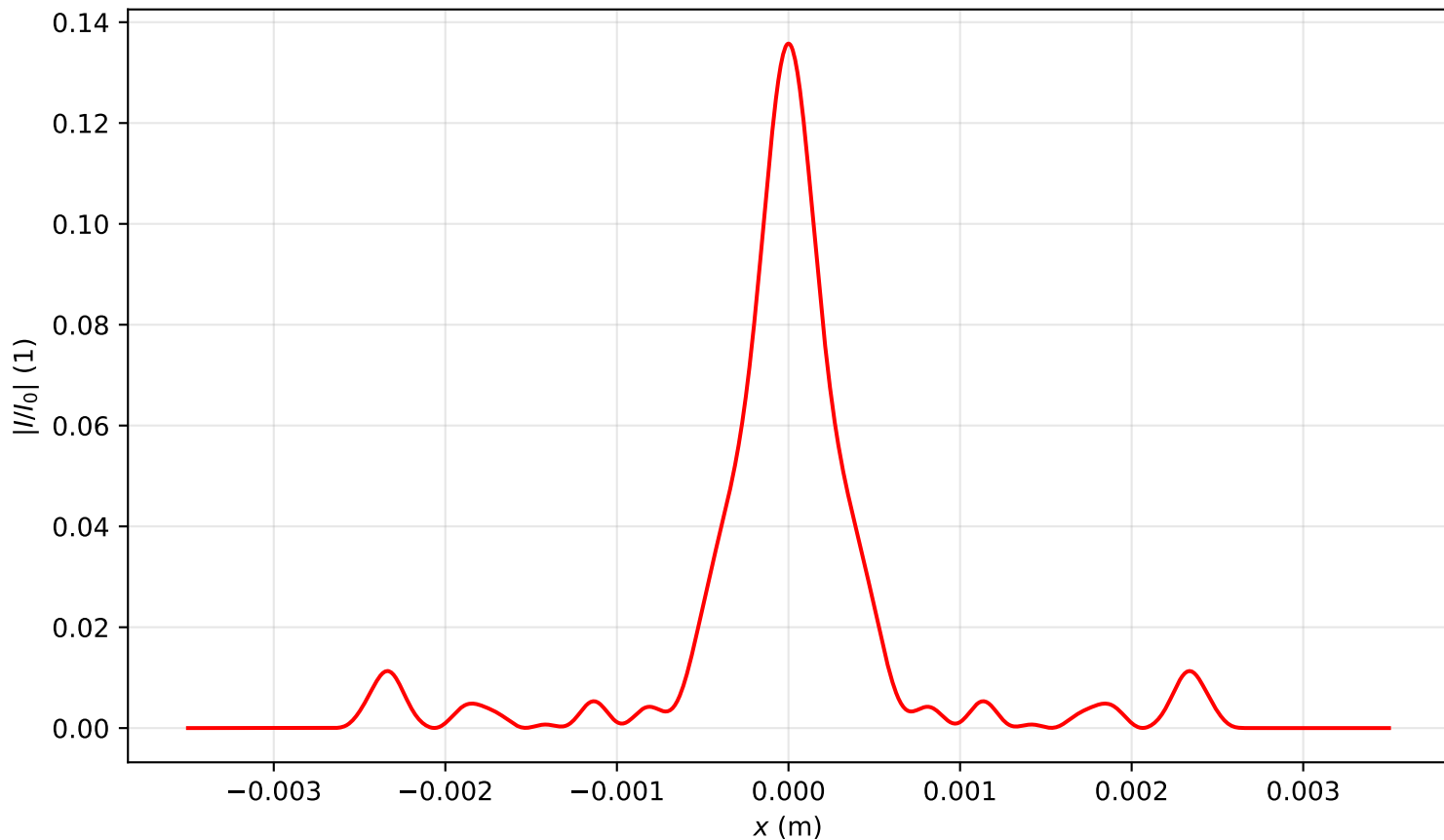
Intensity profile I(x, y = 0, z = 3.344)/I_0 , P_{in}=9.0P_{cr} , artificial time
